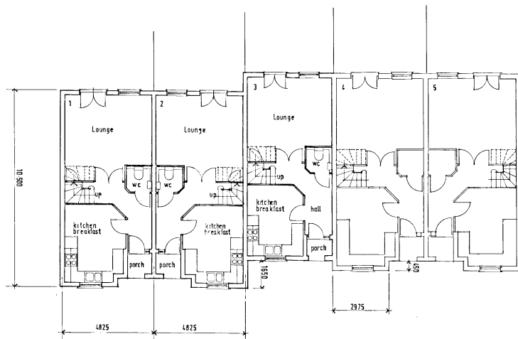
Ground floor plan Gross external floor area: 99.64 m 2 1070 sf 1 Plots 1, 2, 4 and 5 96.98 m 2 1044 sf 1 Plot 3
