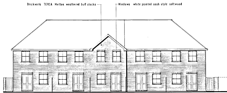
Rear [south] elevation
