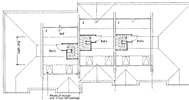
Roof floor plan: Additional floor area: 26.53 m 2 285 sf 1 Plots 2, 3 and 4
