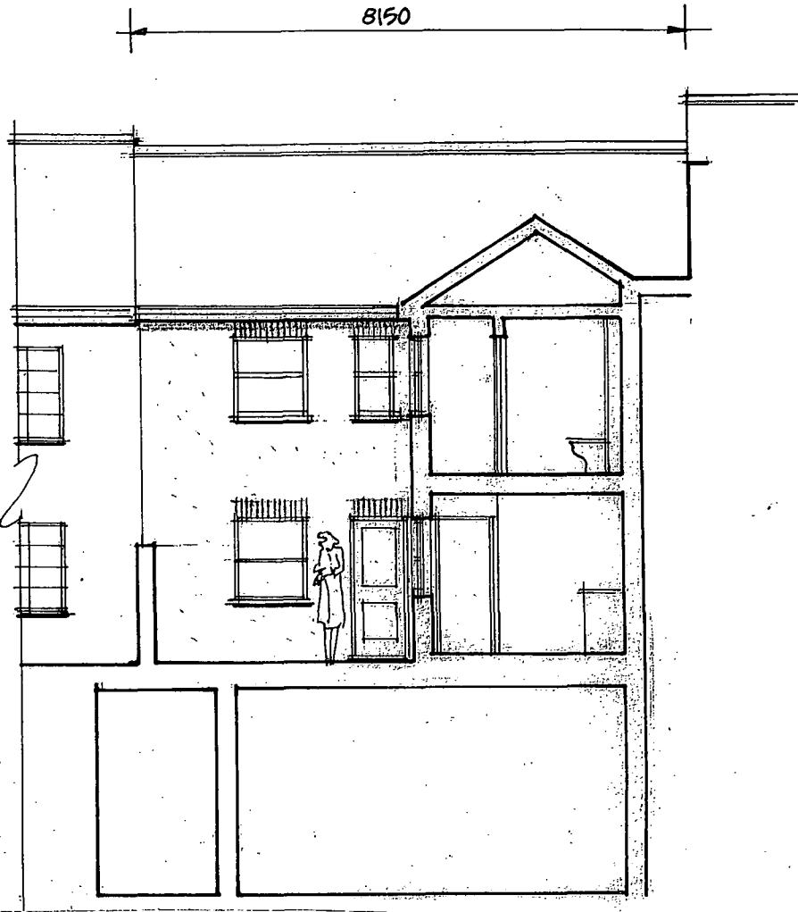
PROPOSED SECTION CC SHOWING REAR ELEVATION ROOF
